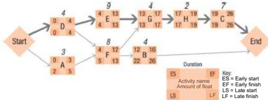
FIGURE 8.13 Backward pass through network diagram
