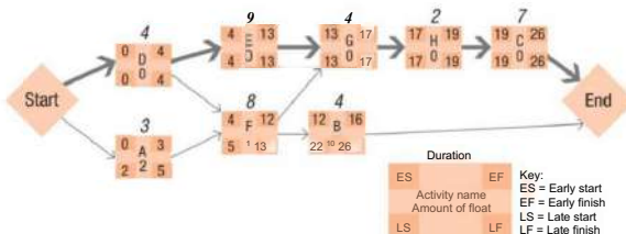
FIGURE 8.14 Float of activities on network diagram
