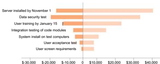
FIGURE 12.6 Tornado diagram
